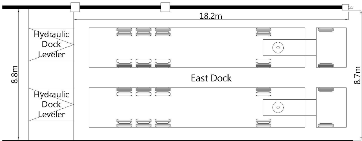
Figure 4.2- East Loading Dock Section
