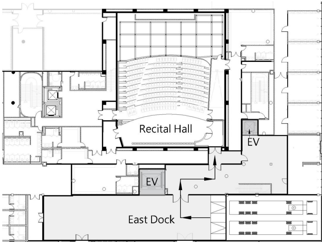
Figure 4.3 - Loading Flow
