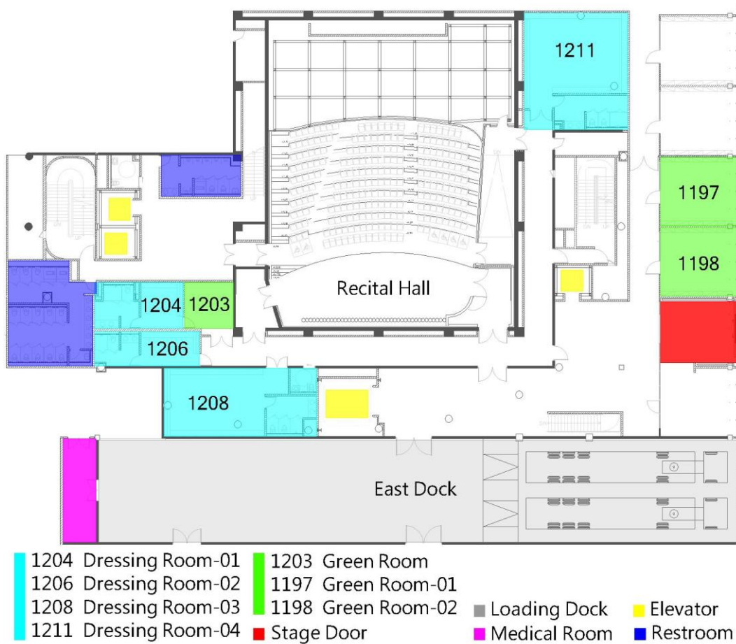
Figure 0.2- Recital Hall Plan
