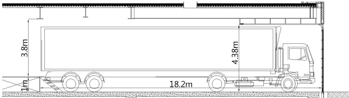
Figure 4.1- East Loading Dock Plan
