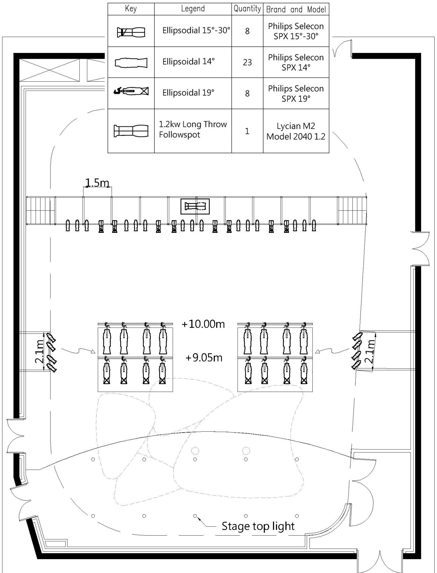
Figure 2.1—Lighting Plan
