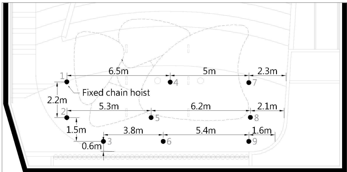
Figure 1.4 - Stage Hoisting plan
